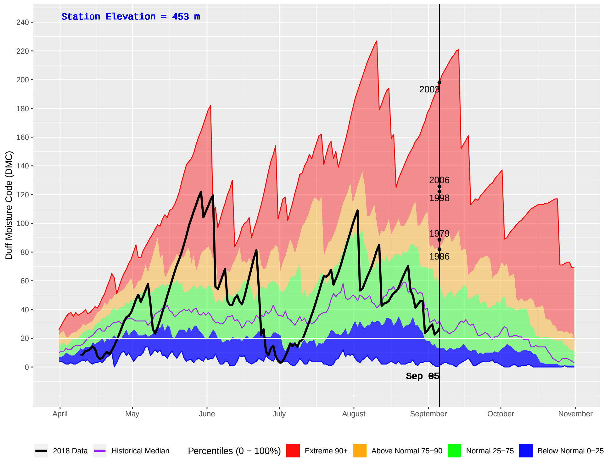
CLEARWATER HUB (239) : Historical (1976–2016) and Current (2018) Daily Duff Moisture Code (DMC)
