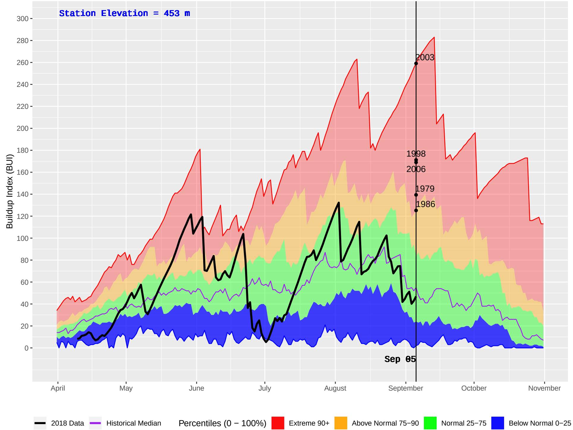
CLEARWATER HUB (239) : Historical (1976–2016) and Current (2018) Daily Buildup Index (BUI)
