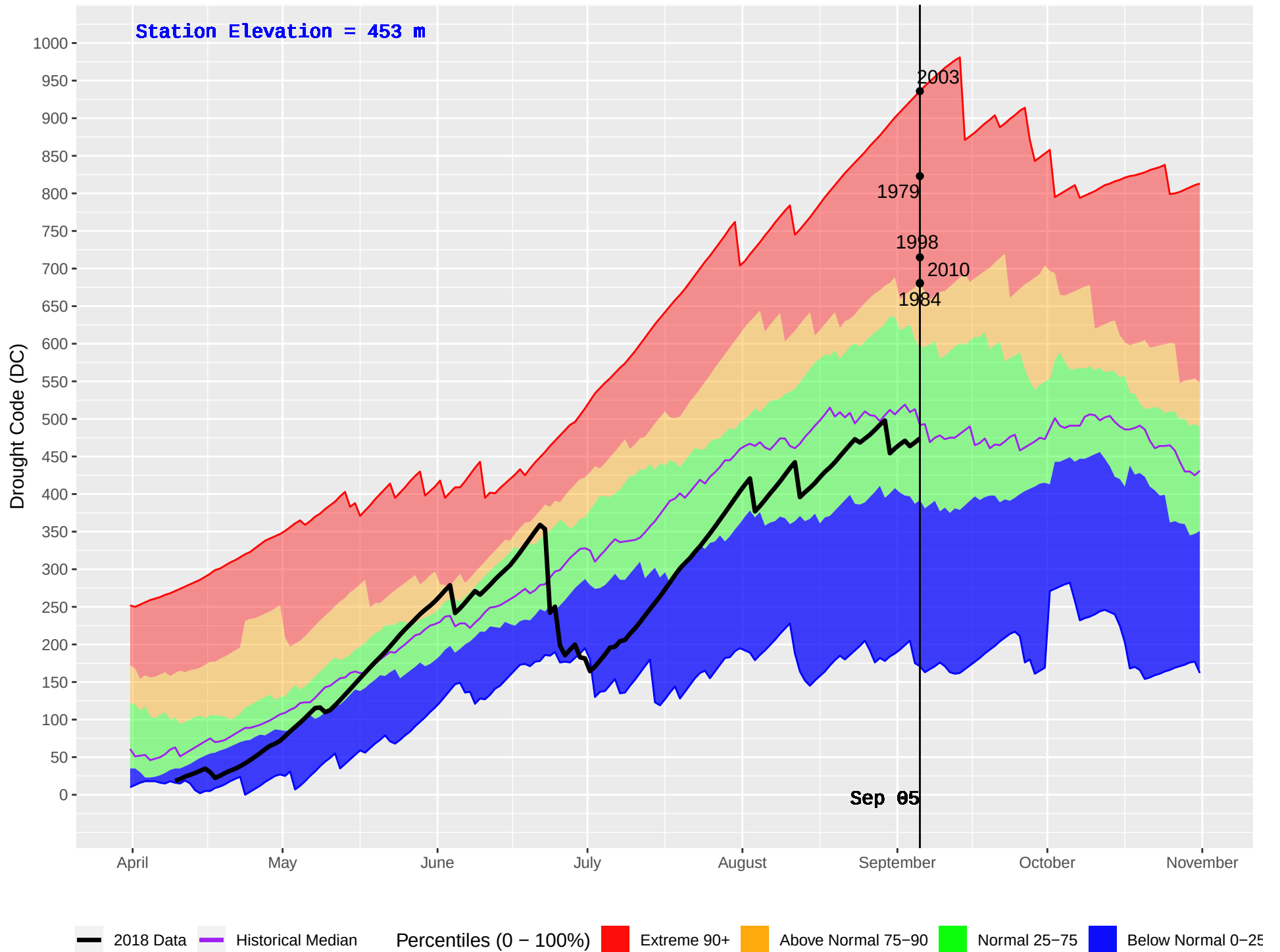
CLEARWATER HUB (239) : Historical (1976–2016) and Current (2018) Daily Drought Code (DC)
