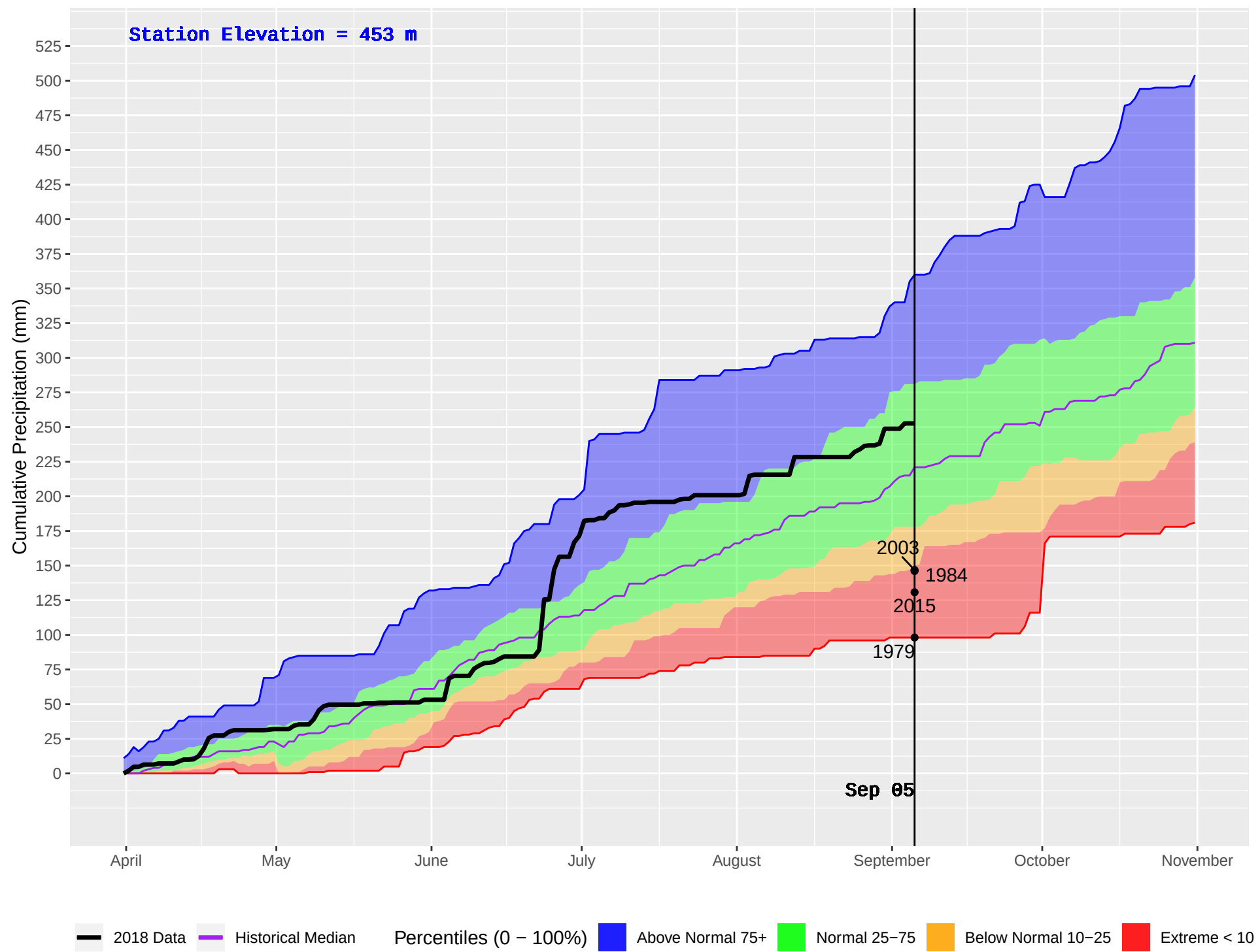
CLEARWATER HUB (239) : Historical (1976–2016) and Current (2018) Daily Cumulative Precipitation
