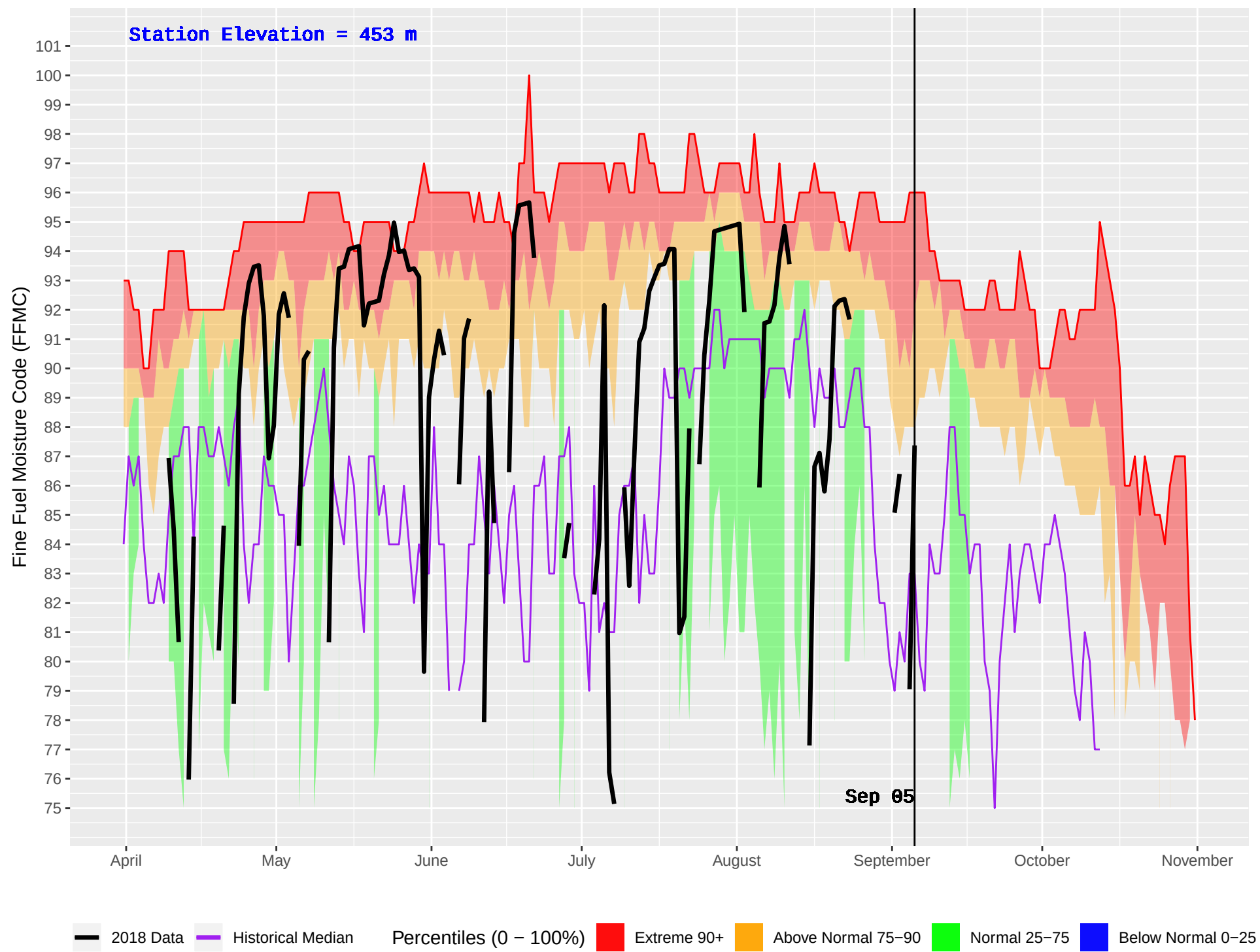
CLEARWATER HUB (239) : Historical (1976–2016) and Current (2018) Daily Fine Fuel Moisture Code (FFMC)
