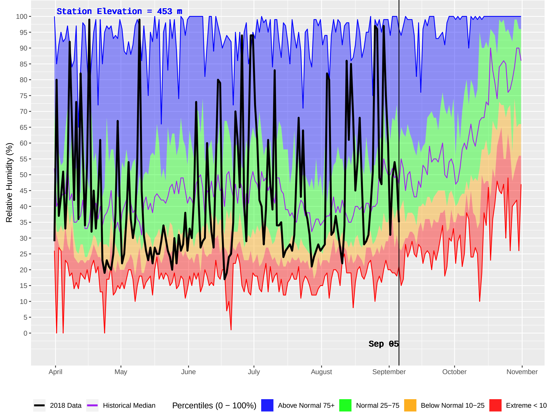
CLEARWATER HUB (239) : Historical (1976–2016) and Current (2018) Daily Relative Humidity
